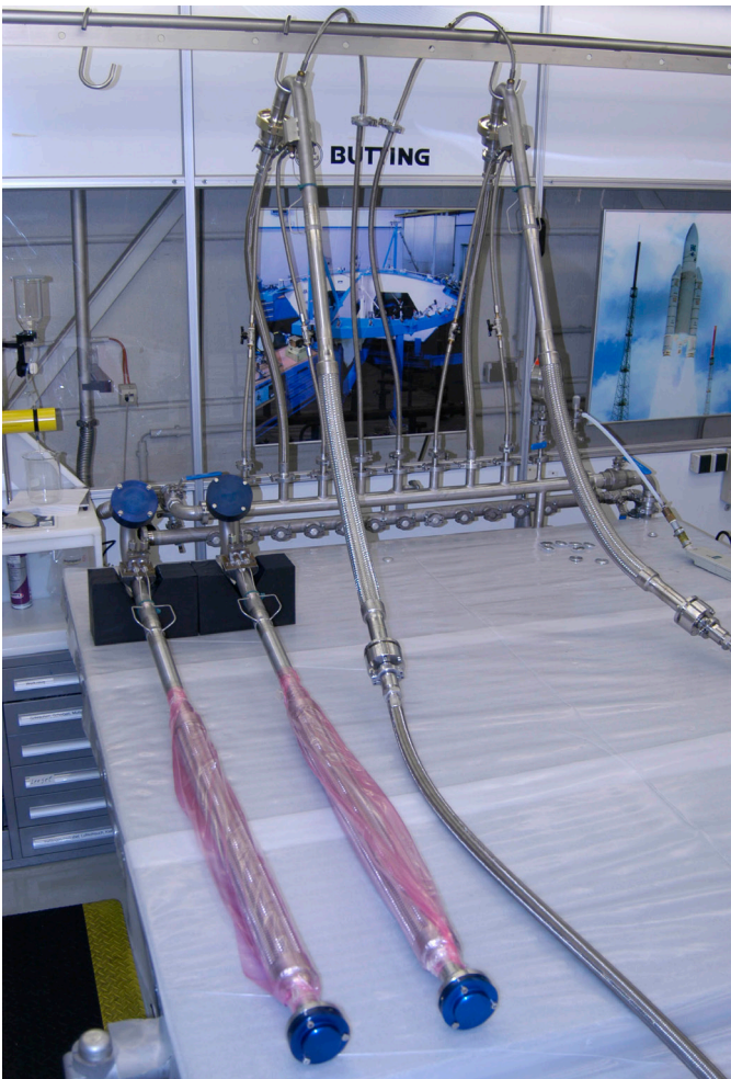
Cleanroom cabin class 100 000 with cleaning system according ARIANE line standard. Example for the final cleaning of oxygen lines etc.
